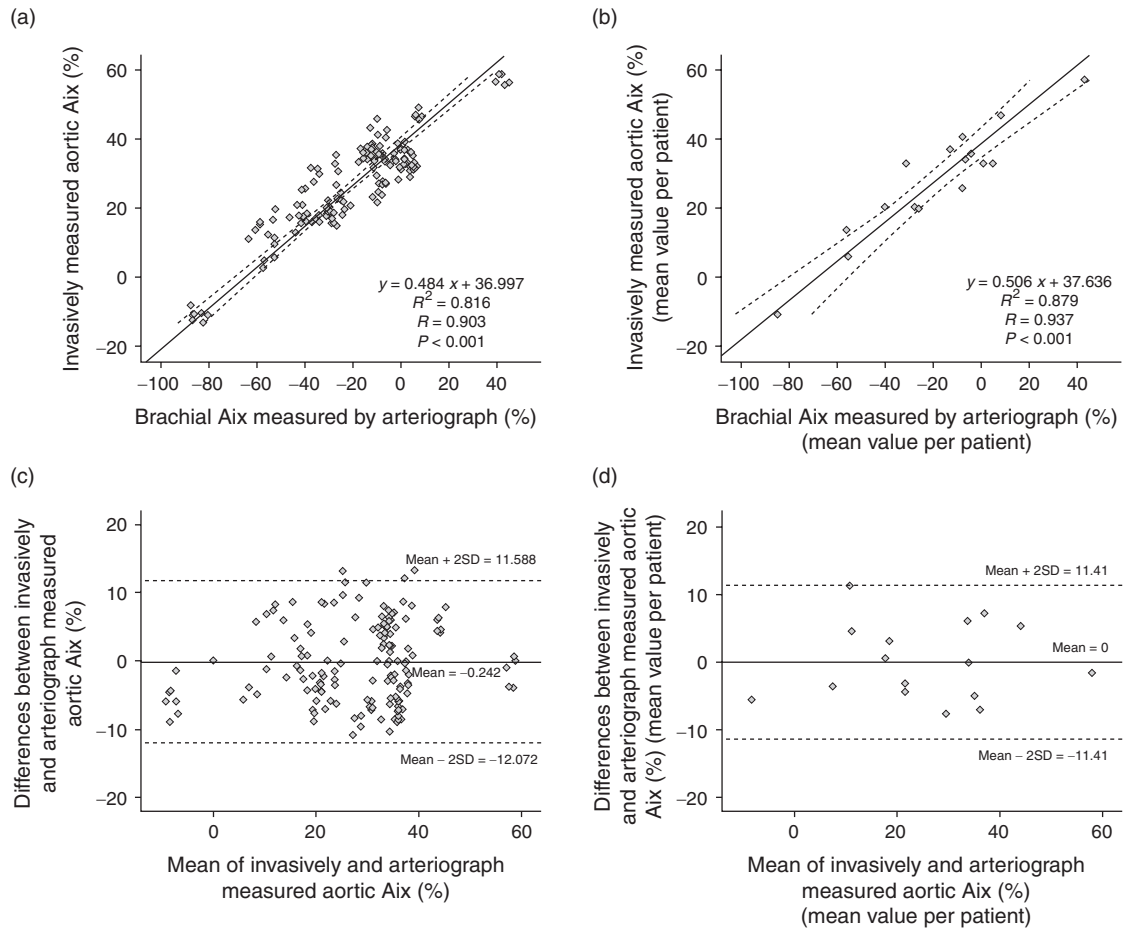
Comparison of intra-aortic and Arteriograph-measured brachial augmentation index. (a) Relationship between brachial Aix measured by Arteriograph and invasively measured aortic Aix (beat-to-beat basis). (b) Relationship between brachial Aix measured by Arteriograph and invasively measured aortic Aix (mean value per patient). (c) Bland–Altman analysis of mean values and differences for aortic Aix measured invasively and by Arteriograph (beat-to-beat basis). (d) Bland–Altman analysis of mean values and differences for aortic Aix measured invasively and by Arteriograph (mean value per patient). Aix, aortic augmentation index.
